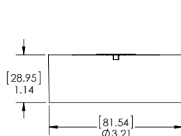
HOUSING (NO GASKET)
